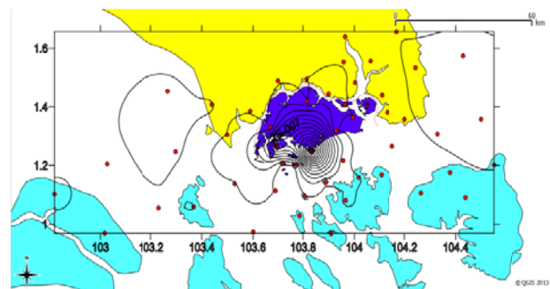
Figure 7: Distribution of AIS Receptor and CO 2 Emission
