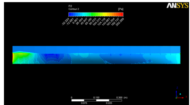
Figure 10(b): Dynamic pressure contours on the Wigley hull at Fr = 0.267 ( V = 0.8363 m/s) for Grid2.
