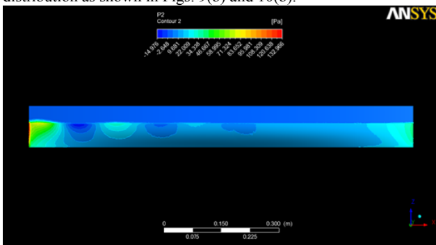
Figure 9(a): Dynamic pressure contours on Wigley hull at Fr = 0.2 ( V = 0.6264 m/s) for Grid1.
