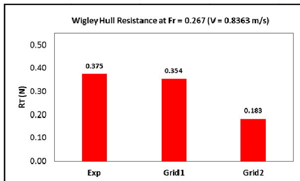
Figure 6: Comparison between Wigley hull experimental [20] and predicted numerical results at Fr = 0.267 ( V = 0.8363 m/s).
