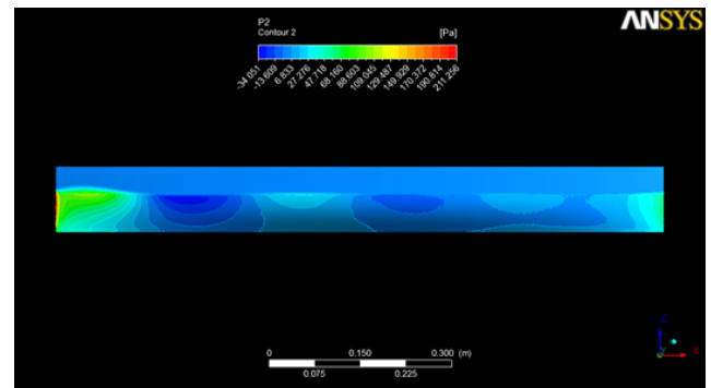
Figure 10(a): Dynamic pressure contours on the Wigley hull at Fr = 0.267 ( V = 0.8363 m/s) for Grid1.
