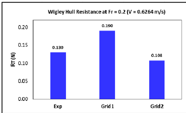
Figure 5: Comparison between Wigley hull experimental [20] and predicted numerical results at Fr = 0.2 ( V = 0.6264 m/s).
