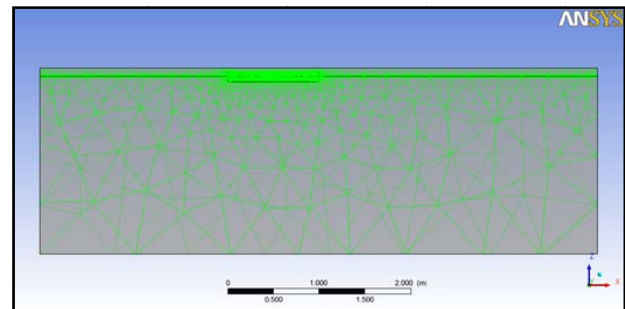
Figure 4(a): Grid2 with prism layers in the free surface region only (total number of mesh elements is 3,731,145 tetrahedral elements)
