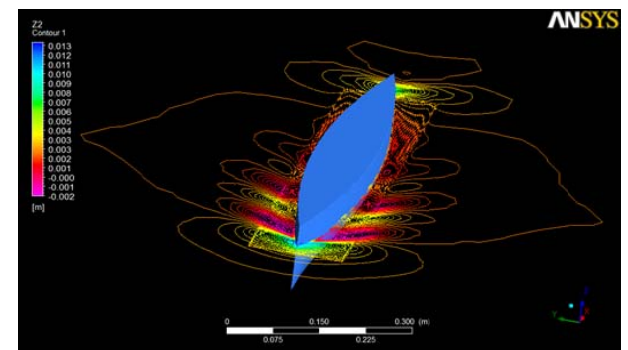
Figure 7(b): Grid2 wave contours around Wigley hull at Fr = 0.2 ( V = 0.6264 m/s).
