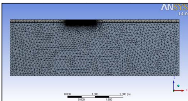
Figure 3(a): Grid1 with prism layers in the free surface region and on Wigley hull (total number of mesh elements is 1,598,573 tetrahedral elements).
