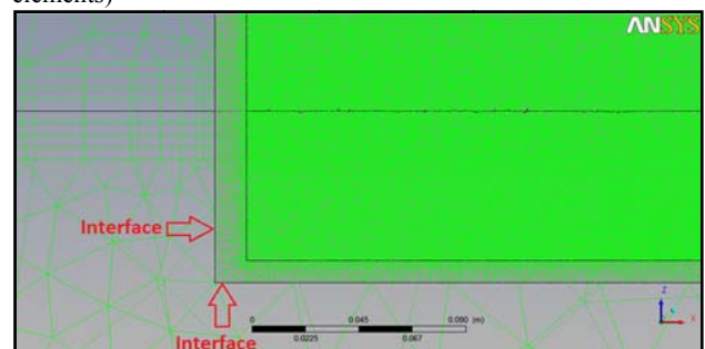
Figure 4(b): Grid2 interfaces plans between the sub-domains. No prism layers in the ship internal domain for the free surface.
