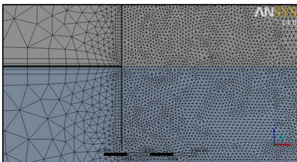
Figure 3(b): Close view for the prism layers on Wigley hull and free surface area for Grid1.
