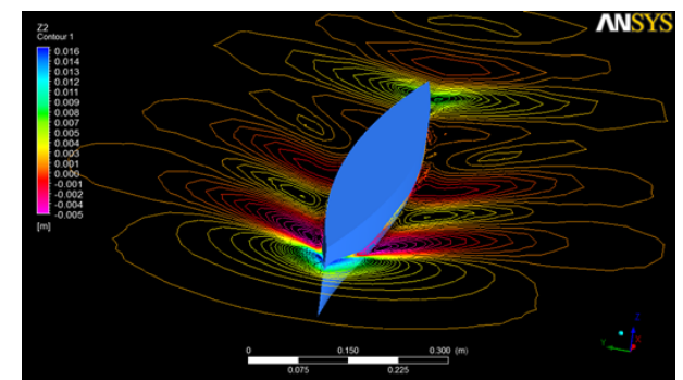
Figure 8(a): Grid1 wave contours around Wigley hull at Fr = 0.267 ( V = 0.8363 m/s).
