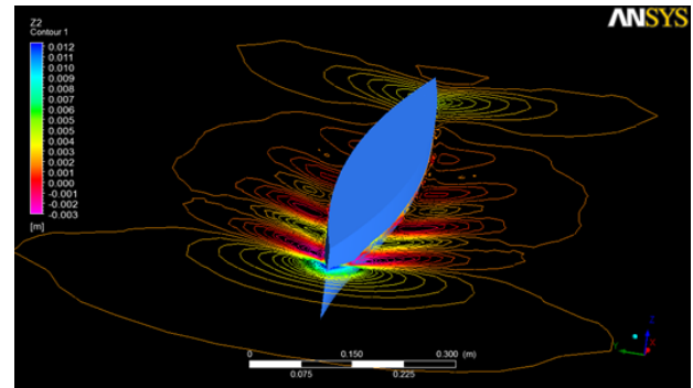
Figure 7(a): Grid1 wave contours around Wigley hull at Fr = 0.2 ( V = 0.6264 m/s).
