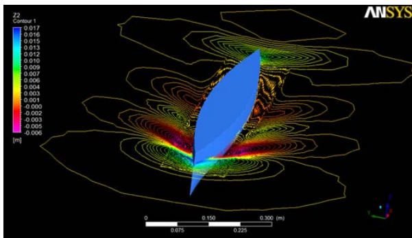
Figure 8(b): Grid2 wave contours around Wigley hull at Fr = 0.267 ( V = 0.8363 m/s).
