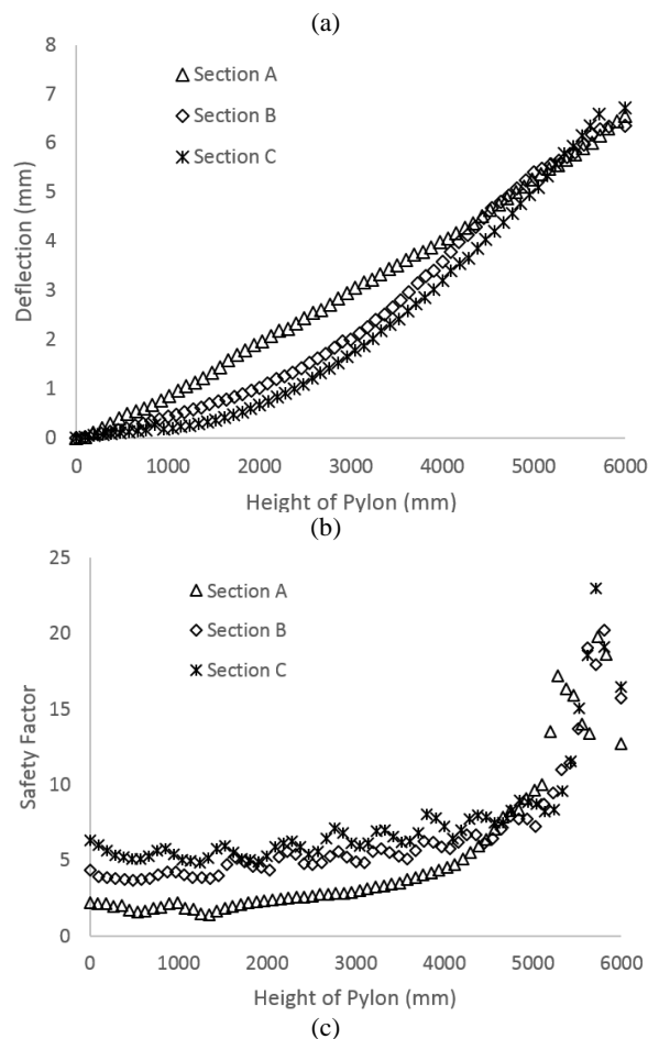
Figure 9: Distribution along longitudinal axis of pylon for: (a) stress, (b) deflection, and (c) safety factor
