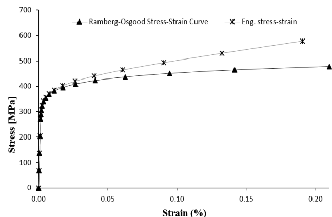
Figure 2: True stress-strain curve of pylon material which is
