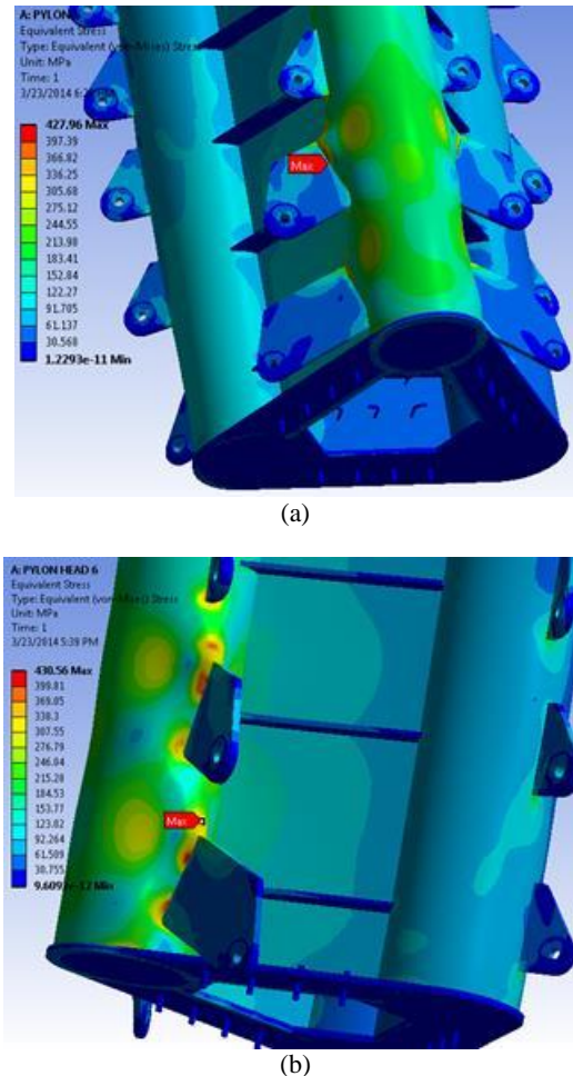
Figure 6: Stress distribution at bottom side of pylon: (a) left side pylon, (b) right side pylon
