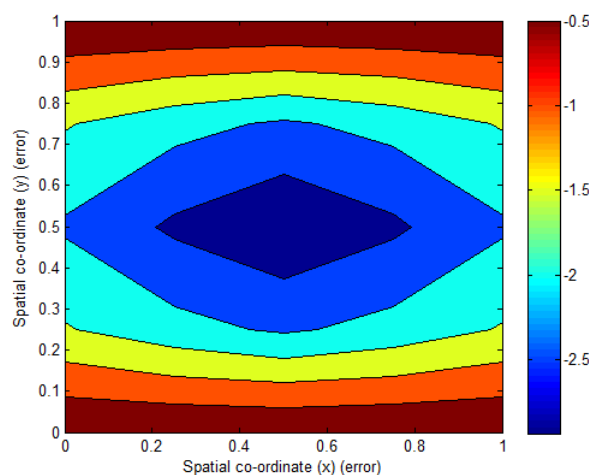
Fig. 3. Error of heat distribution of two-dimensional regular geometry heat transfer problem using FDM.
