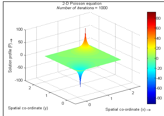
Fig. 2. Solution of heat distribution of two-dimensional regular geometry heat transfer problem using FDM when step size = 100.
