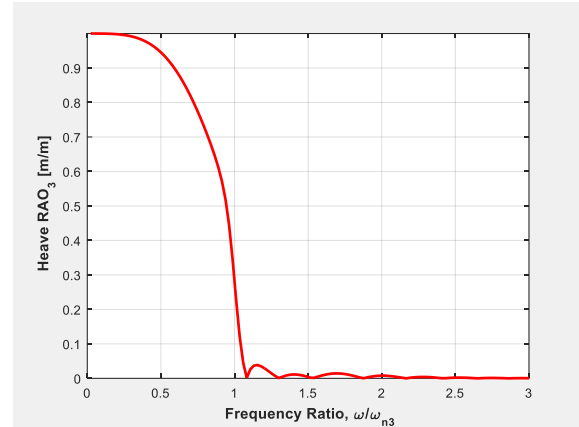
Figure 1: Heave response varying with wave frequency
