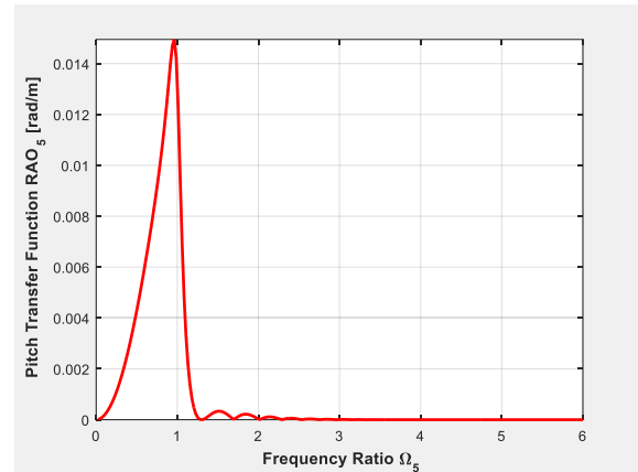
Figure 2: Pitch response varying with wave frequency
