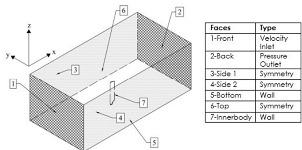
Figure 9 Boundary conditions of 3D block geometry
