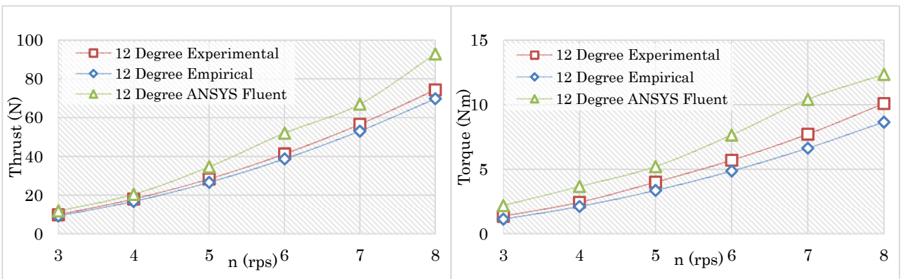
b) 12° Angle of Attack (AOA)
