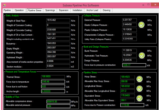
Figure 8: Collapse, burst and stress of subsea Pipeline
