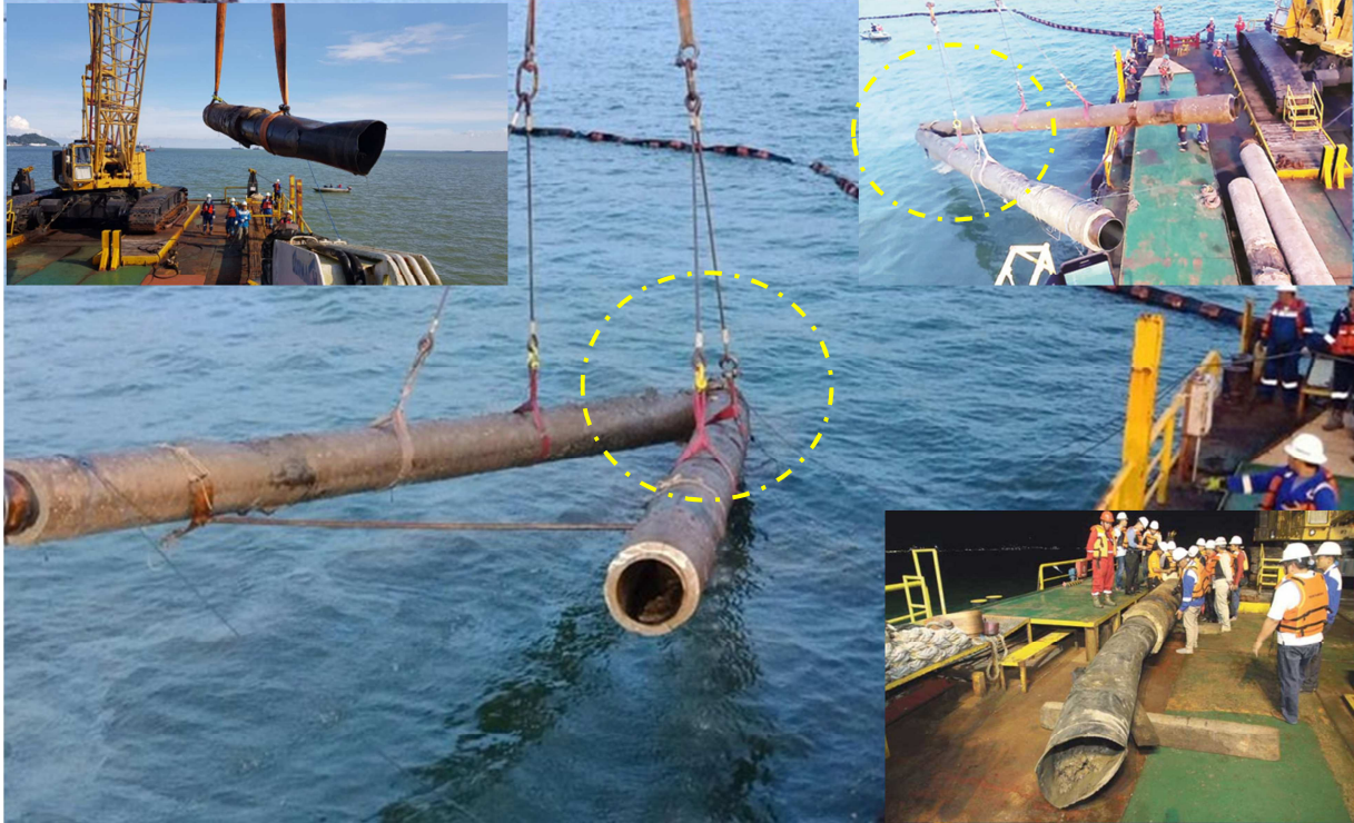
Figure 11: Lifting of subsea pipeline from Sea Heaven.
