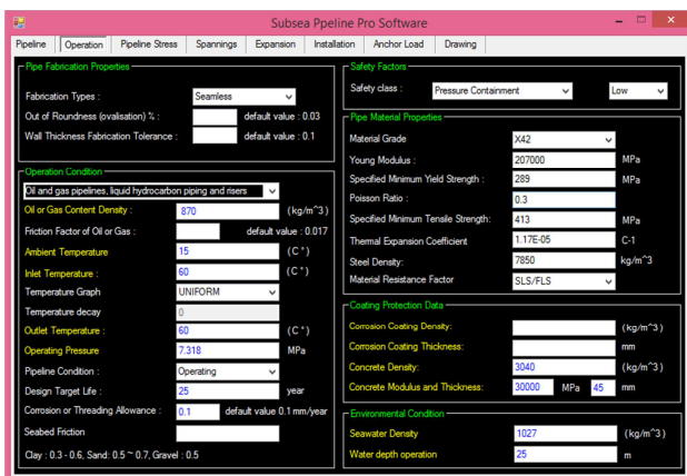
Figure 7: Operation, material properties and environmental data
