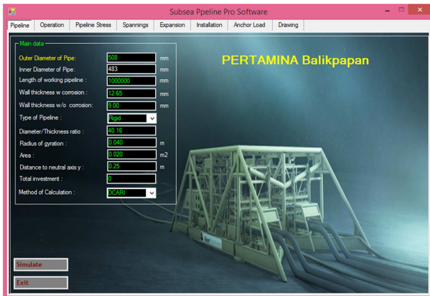
Figure 6: Main principal data of subsea Pipeline
