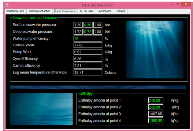
Figure 8.d: Cycle performance of OTEC.
