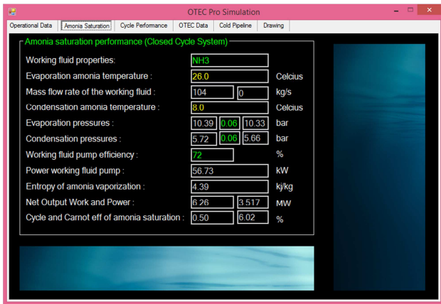
Figure 8.c: Ammonia saturation of OTEC.
