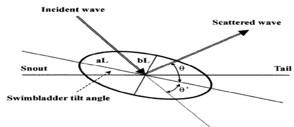
Figure 7: Swim bladder Geometry for Soft spheroid models
