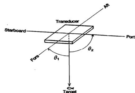
Figure 4: Geometry targets in Split Beam transducer. Towards the target defined by the \theta_1 and \theta_2 angle
