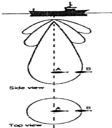
Figure 5: The working principle of Split Beam on detecting fish echo sounder.
