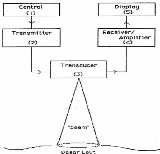
Figure 1: Working mode of hydroacoustic tool
