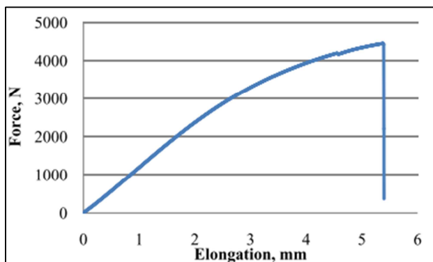
Figure 10: Tensile test result of 2.5mm nominal diameter steel wire rope
