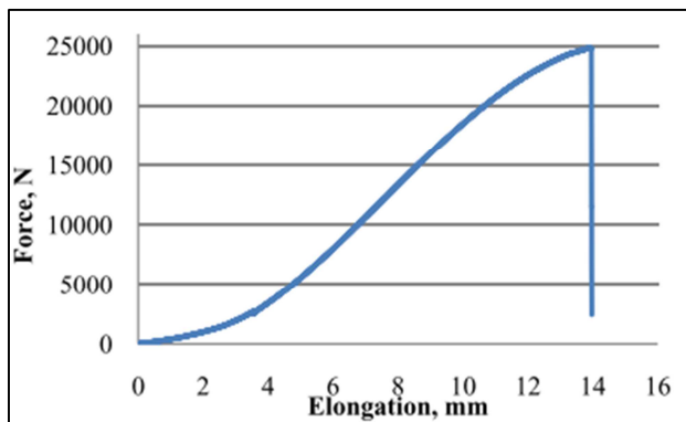
Figure 11: Tensile test result of 6mm nominal diameter steel wire rope
