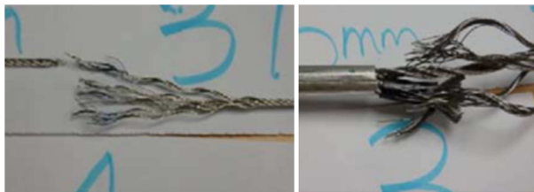
(2.5mm wire rope) (6mm wire rope) Figure 9: Tested wire rope samples
