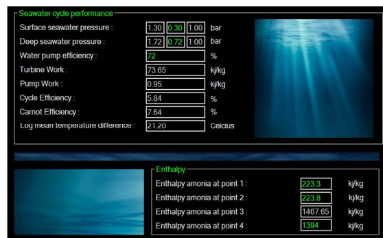
Figure 4.3: Result simulations in OTEC Pro
