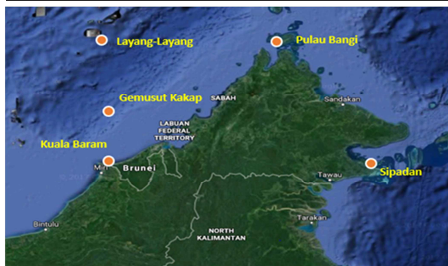
Figure 2.3: Potential sites of OTEC in Malaysia
